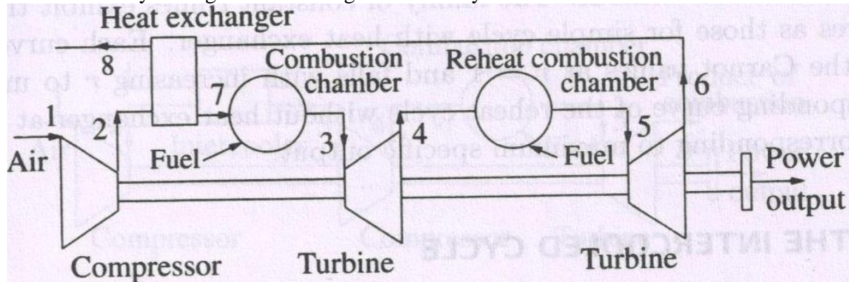
Fig. 47. Arrangement of reheat cycle with heat exchanger
