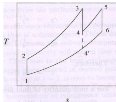
T-S diagram
