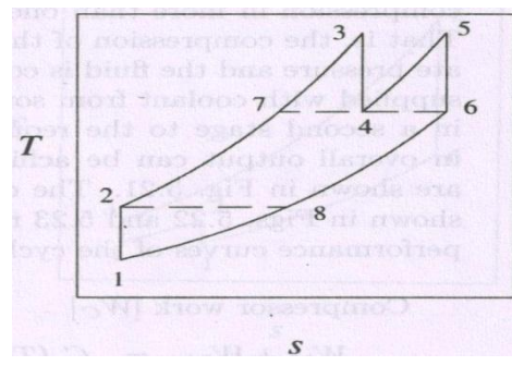
T-S diagram
