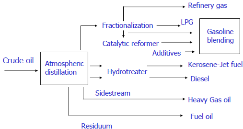
Fig. 10. Refinery processes
